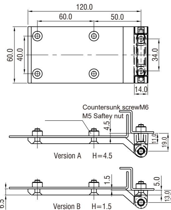
Screw-on hinge zinc die, pin stainless steel and bush polyamide
