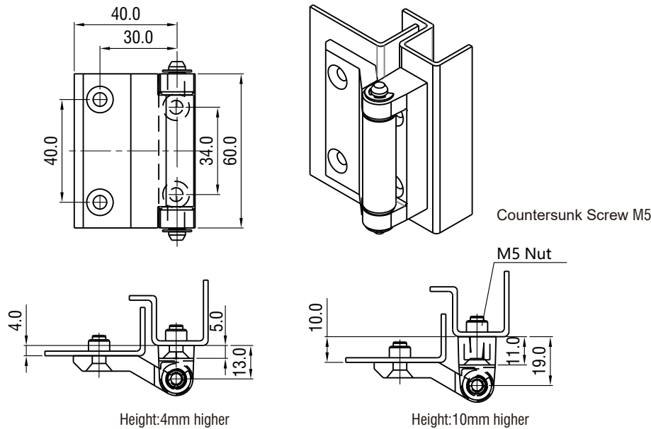
Screw-on hinge zinc die, SUS pin
