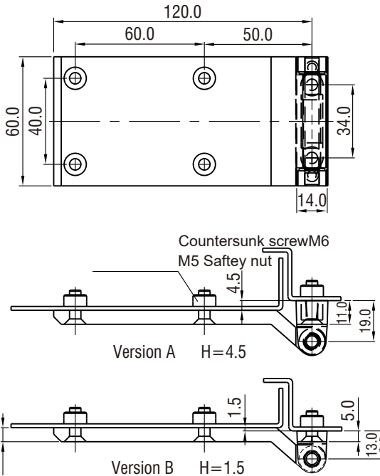
Screw-on hinge zinc die, pin stainless steel and bush polyamide
