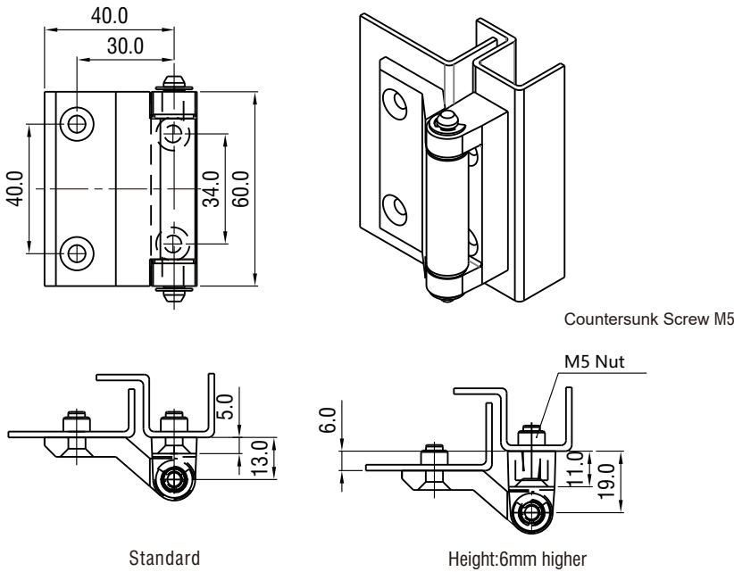
Screw-on hinge zinc die, SUS pin
