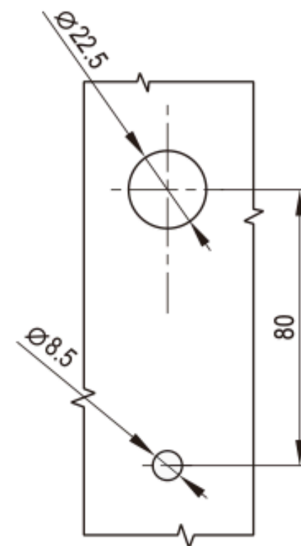
Panel Cutout
