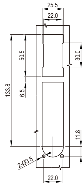
Panel Cutout
