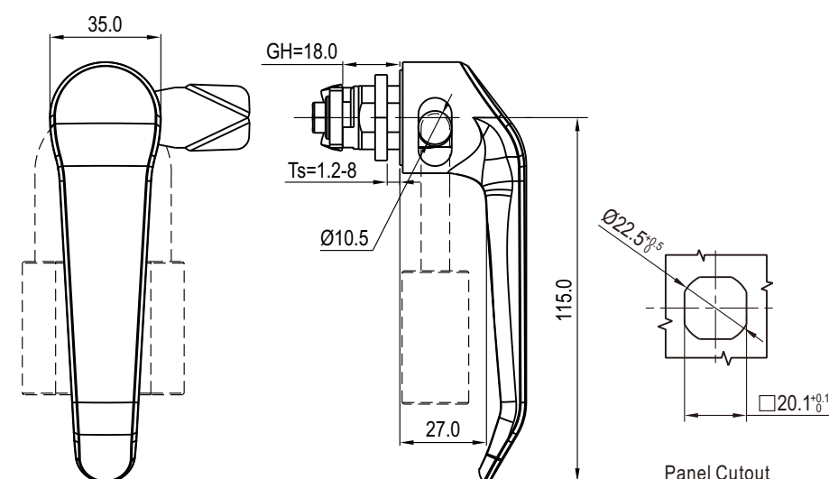
Panel Cutout
