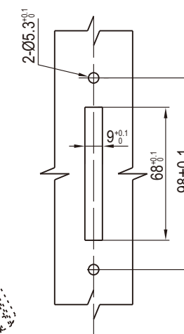
Panel Cutout
