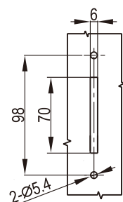
Panel Cutout
