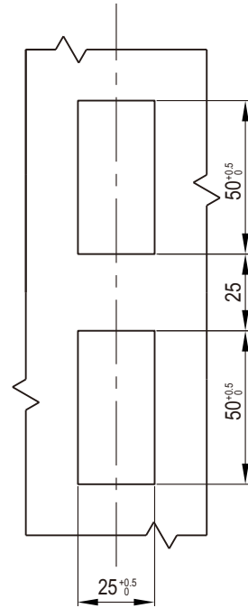
Panel Cutout
