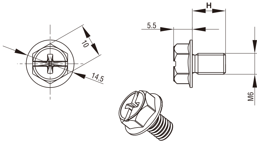
External hexagonal cross flange screw
