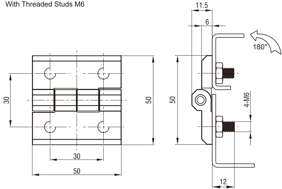
With Threaded Studs M6
