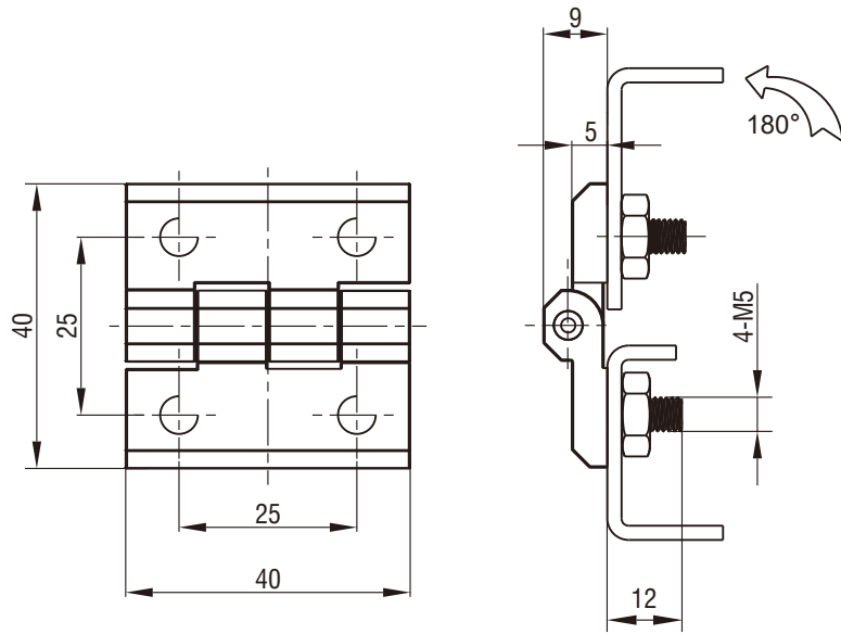
With Threaded Studs M5
