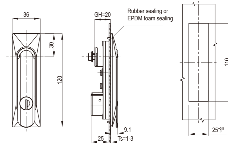
Panel Cutout
