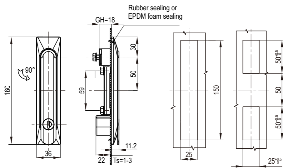
Panel Cutout
