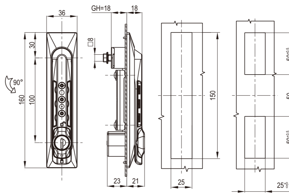
Panel Cutout
