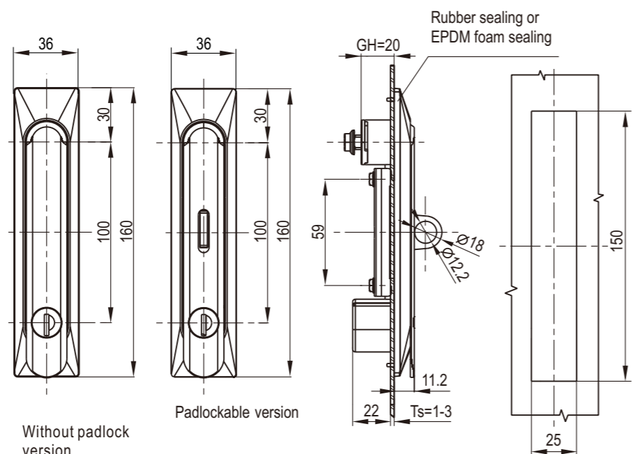
Panel Cutout
