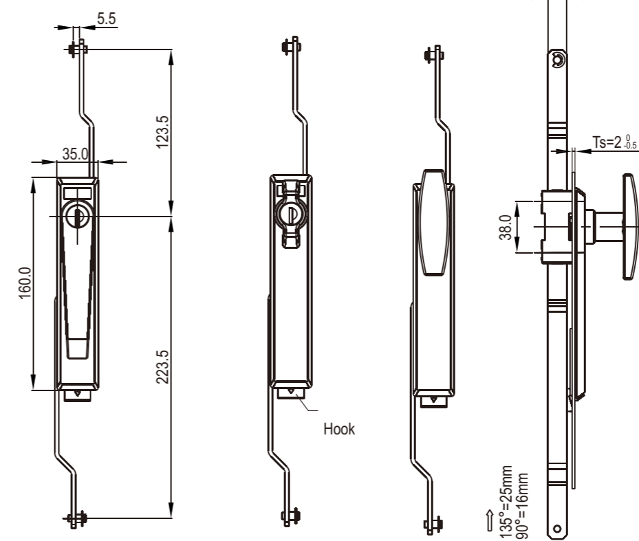
Rod control
