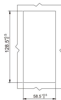
Panel Cutout
