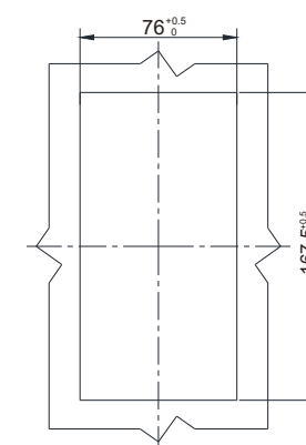
Panel Cutout
