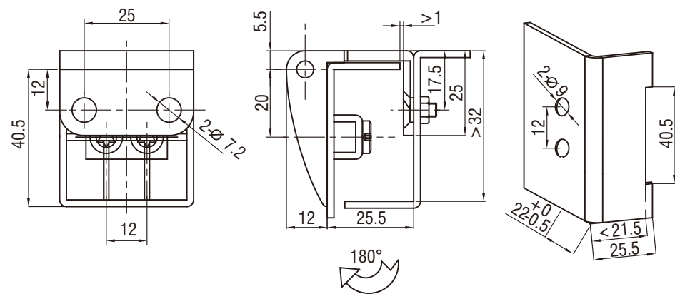
Panel Cutout
