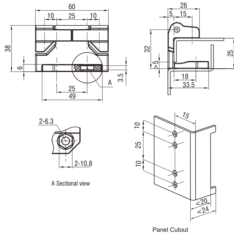
Panel Cutout
