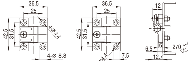
Round screw hole
