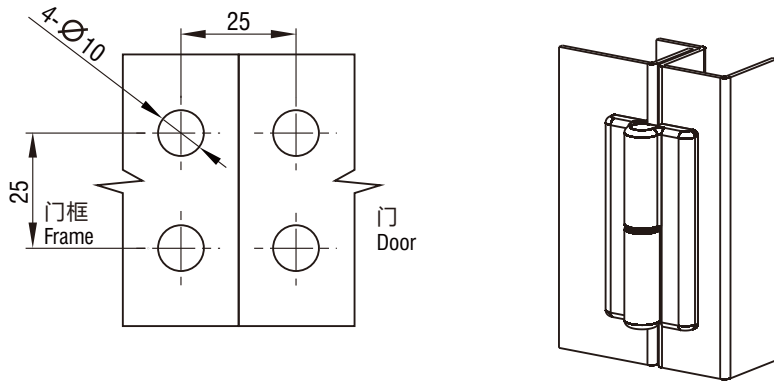
Panel Cutout
