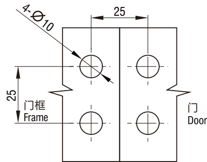
Panel Cutout
